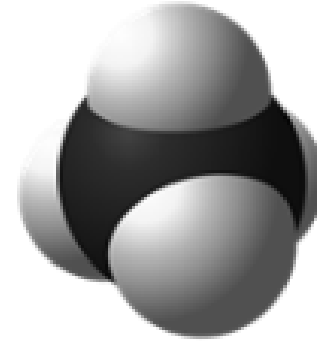
Methane - CH 4
